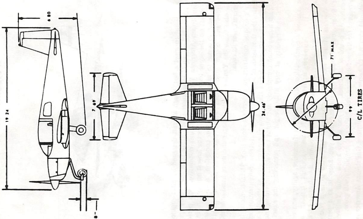
Figure 1. Yankee's principal dimensions.
