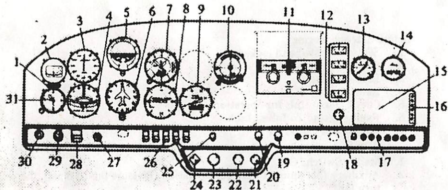
Figure 6. Yankee instrument panel diagram.
